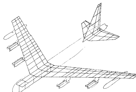
Fig. 2 Doublet lattice aerodynamic paneling.
