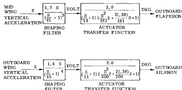
Fig. 6 FMC predicted flutter speed improvement.
