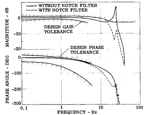
Fig. 13 Outboard aileron ground test frequency response.
